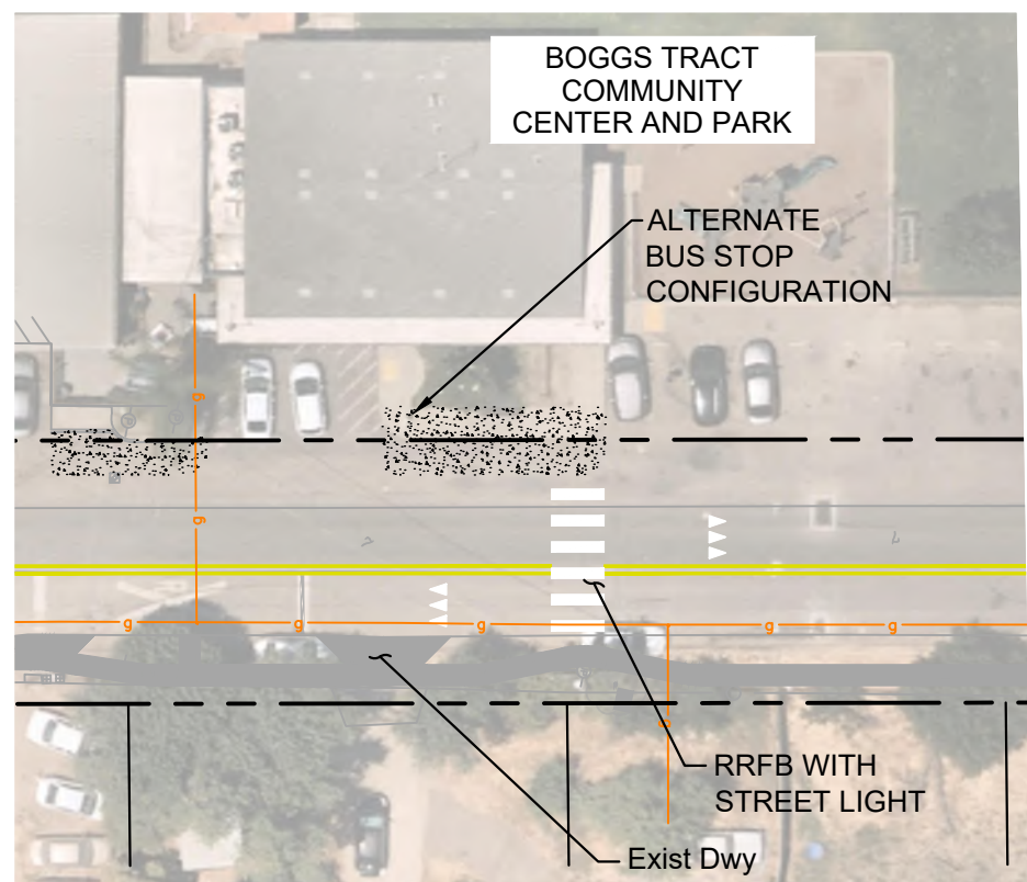
ALTERNATIVE BUS STOP CONFIGURATION
