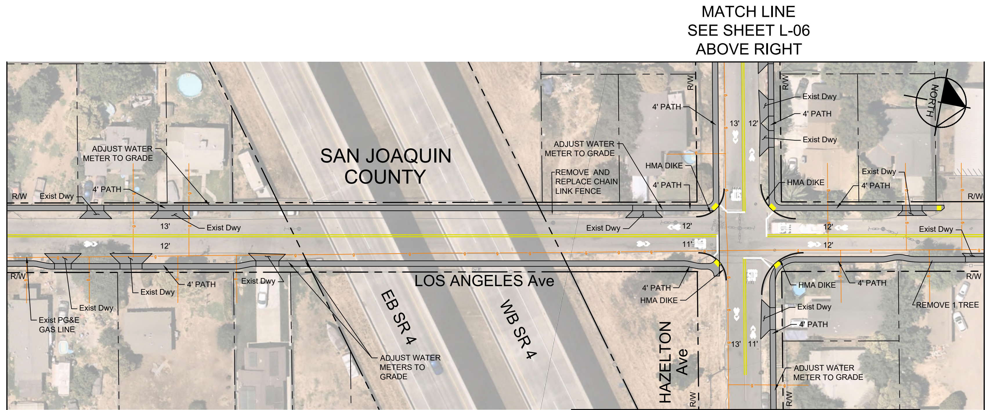
MATCH LINE SEE SHEET L-08 ABOVE RIGHT MATCH LINE SEE SHEET L-06 BELOW LEFT LOS ANGELES AVENUE
