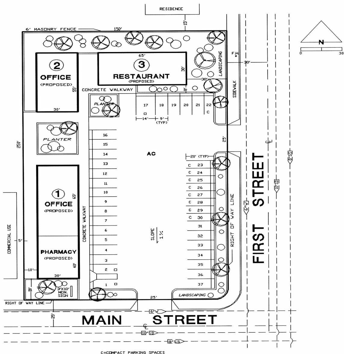
C=COMPACT PARKING SPACES
