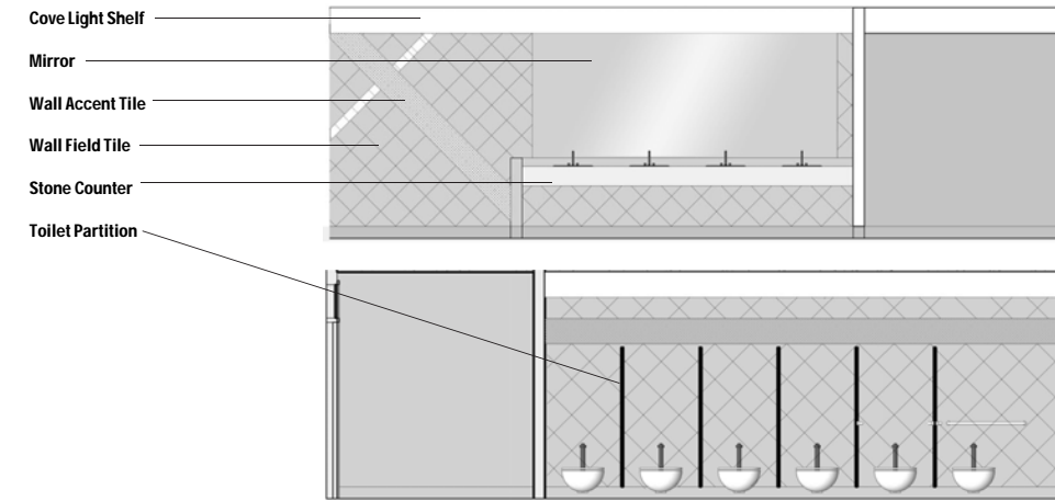
Restroom Elevations
