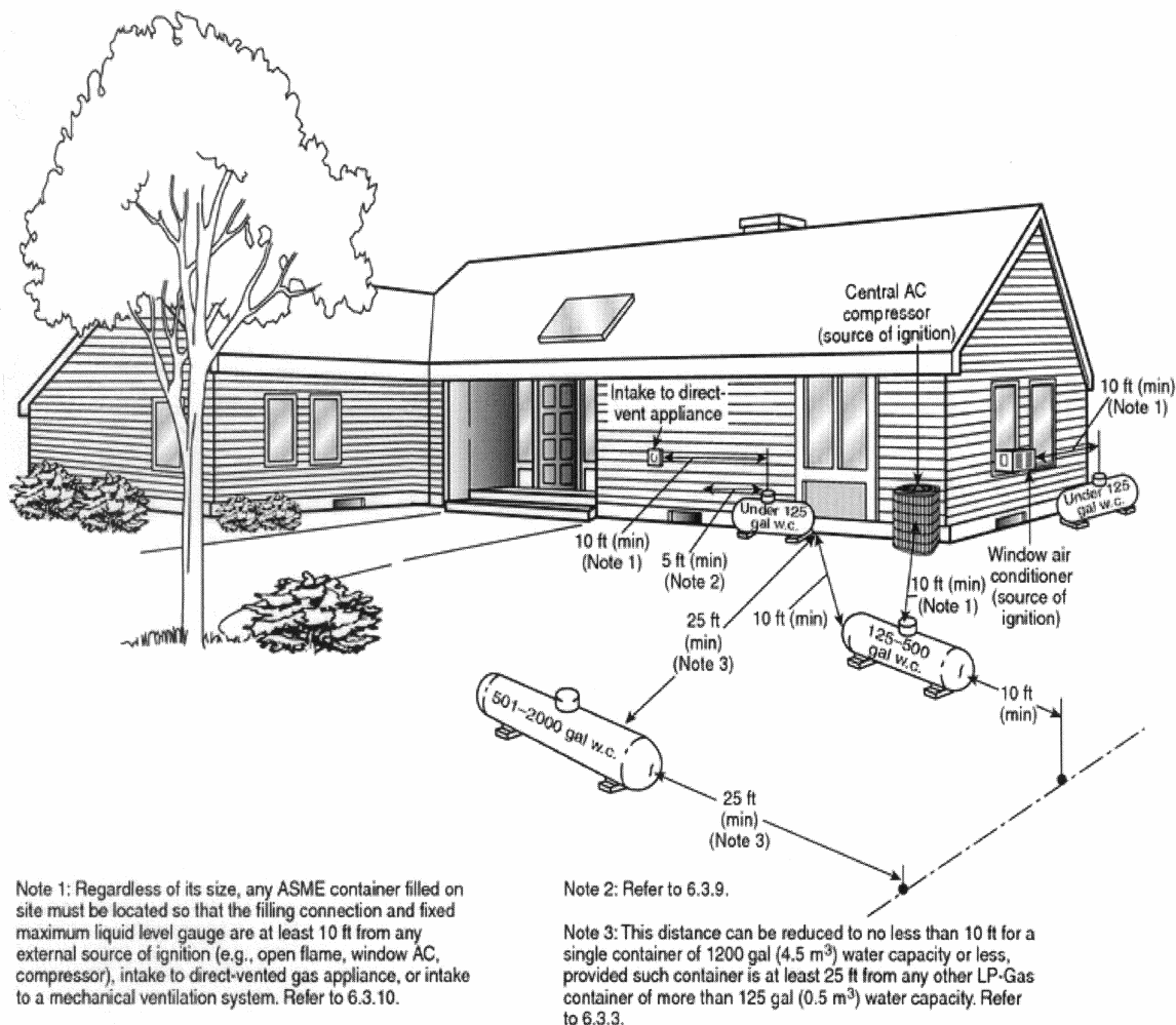
FIGURE I.1(b) Aboveground ASME Containers. (This figure for illustrative purposes only; code shall govern.)
