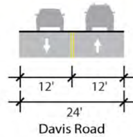
EXISTING TYPICAL SECTION
