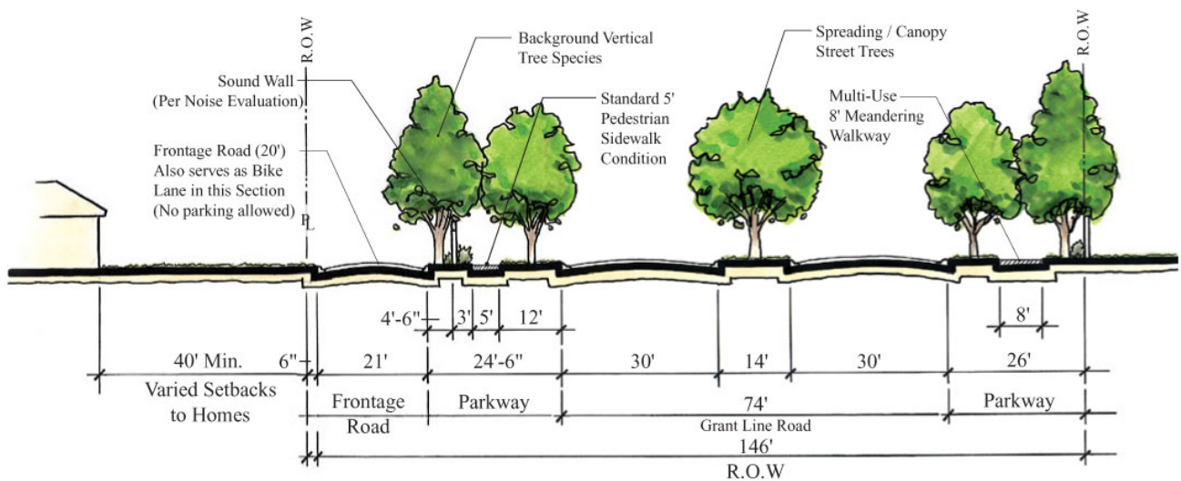
Grant Line Road Typical Cross Section
